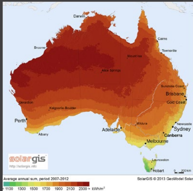
Global Horizontal Irradiation, Australia
